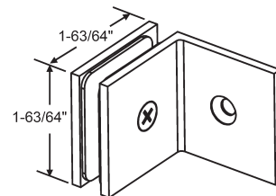
Brass shower glass clamp, clear PVC gasket. Includes Philips screws, Allen screws and Allen key. Wall to glass 90°, with large leg. Suitable for glass 8 - 12 mm
