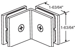
Solid brass shower glass clamp, clear PVC gasket. Includes Philips screws, Allen screws and Allen key. Glass to glass 90° Suitable for glass 8 - 12 mm.
