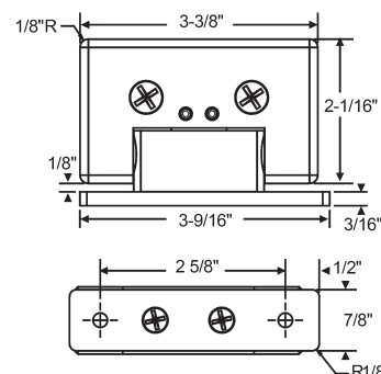
Adjustable Bottom Pivot Hinge Radius Corners & Chamfered Edges
