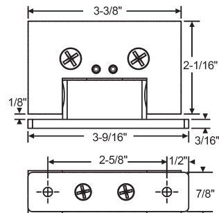
Adjustable Bottom Pivot Hinge Solid Brass
