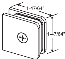
Brass shower glass clamp, clear PVC gasket. Includes Philips screws, Allen screws and Allen key. Wall to glass, hole-in-glass style. Suitable for glass 8 - 12 mm.
