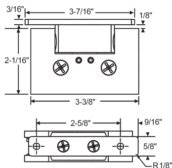
Adjustable Solid Brass Top Pivot Hinge Solid Brass
