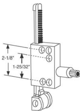
823P Wide Head Tapped Operator 1 Per Bag
