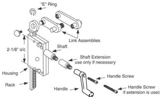
800PK Operator Kit 1 Per Bag
