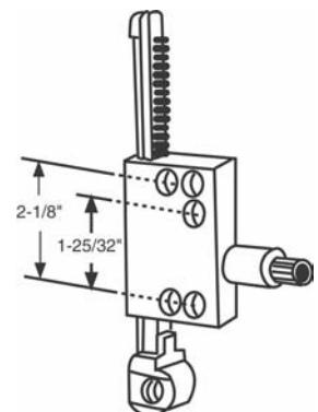
819P Face Mount Rack Operator 1 Per Bag
