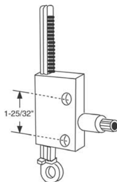
801P Standard Rack Operator 1 Per Bag
