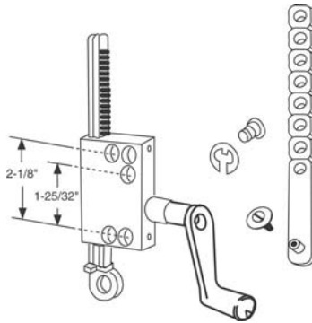
816P Non-Handed Rack with Tapped Holes Operator Kit 1 Per Bag
