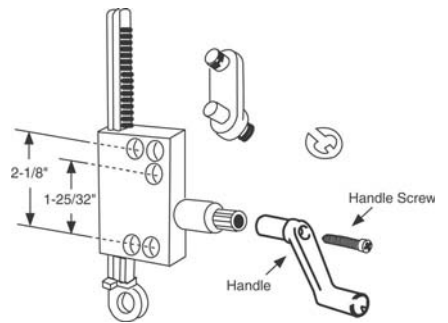
824P Rack Operator with Link 1 Per Bag
