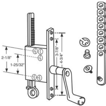
815P Face Mount Rack Operator 1 Per Bag
