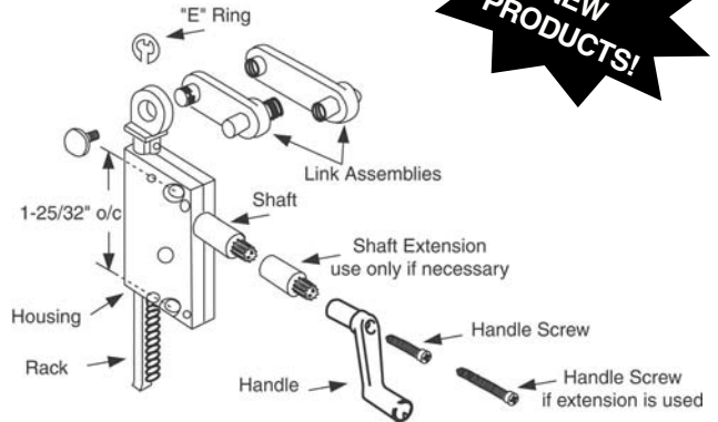
801PK Operator Kit 1 Per Bag
