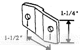
91-70 For plastic laminated panel. 4 required per panel
