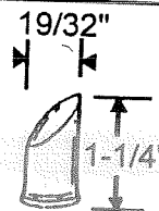
91-114 White Plastic Fits Bracket 91-153 for 7/8" thick doors
