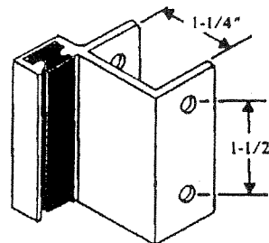
91-78 For plastic laminate pilaster with surface slide latch.
