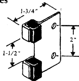
91-88 For any thickness pilaster
