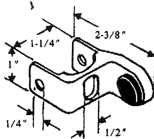
91-87 For steel pilaster with concealed latch.
