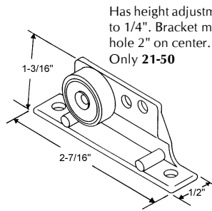
21-57 With 21-50 Roller 21-58 With 21-51 Roller Die Cast
