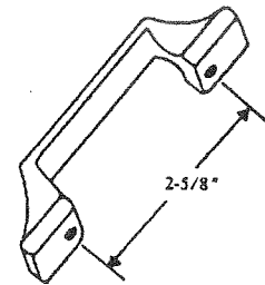
91-90 Mounting Holes Tapped 10-24
