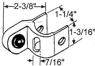
91-5 For steel pilaster with concealed latch.
