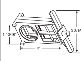
91-129 Zinc Die Cast - Unplated
