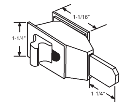
900-18069 With Indicator. For 1" Steel Door
