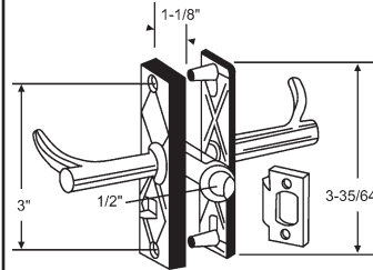
Storm & Screen Latch without Key
