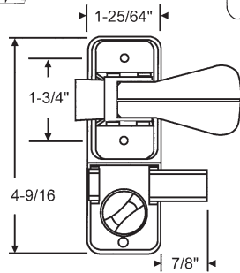
Inside View
