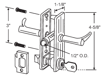
Storm & Screen Latch with Key
