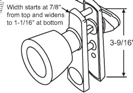
Tulip Knob Latch "No Lock Out" Feature
