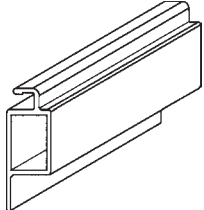
90-1048 (3/8" x 3/4" Box x 5/16" Flange) For Exterior Application
