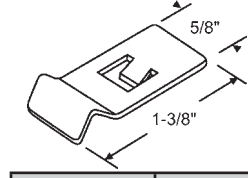
Part # Color 90-715 Bronze 90-715W White 90-715M Mill
