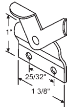
Part # Hand 90-488LH Shown 90-488RH Opposite 1/8" Offset
