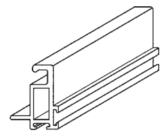
90-1033 (5/16" x 3/4" Box) w/Stopleg & Woolpile
