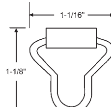
90-104 Small Loop Latch. Used with Ball Head Screw 20-019
