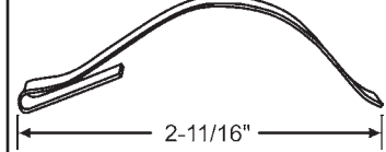
90-628 Tension Spring 1/4" Wide
