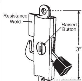
16-673 Raised Button. Front Surface Mounted Steel Hook Peachtree
