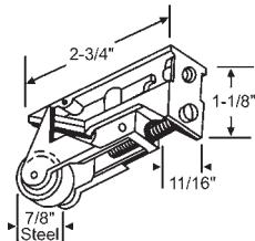
9-303 Flat Roller, Die Cast
