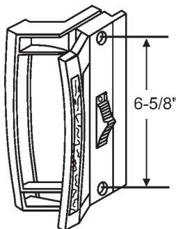
900-16317 Black. Includes Keeper and Screws Norandex
