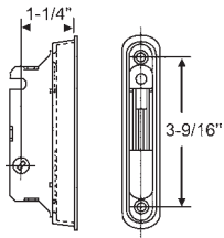
16-443 Mortise Lock and Plate
