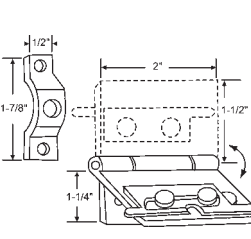
16-406 Aluminum Flip Lock
