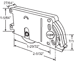
10-443 1" Metal Wheel. Adjustable Vertical Roller 15/64" thru 7/8" Highest Position Norco
