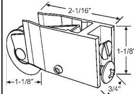
900-11663A with Corner Housing and Screw. Silverline
