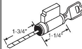
16-133 Key Cylinder Lock
