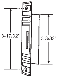
14-151BR Inside Screen Pull Handle. Brown
