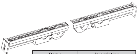
Assembly has Four 1-1/8" Steel Adjustable Rollers-
