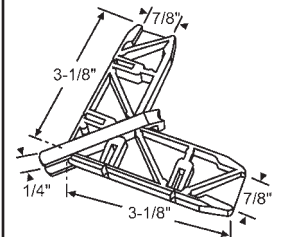
16-361PW White Nylon Miter Corner Use on Door 991M-999
