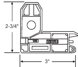
16-116-2 Screen Corner Bracket Assembly with Screw. 2 per Pack
