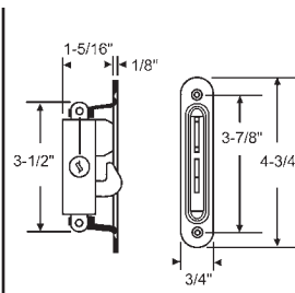
900-9169 Diagonal Hub. Aluminum Finish
