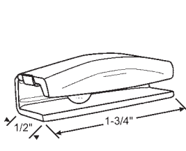
900-10574 Snap-on Vent Lock
