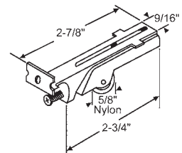
9-202 Flat Roller
