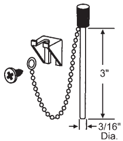
16-104 Burglar Pin/Nite Lock
