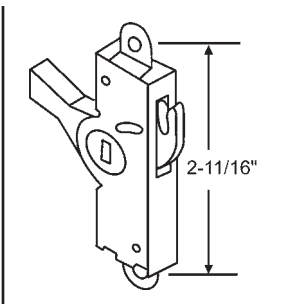
16-142 Used for Surface Mounted Patio Door Handle
