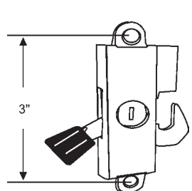
900-7305 Flush Button. Front Surface Mounted Steel Hook Peachtree
