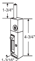
16-687 Security Lock. Aluminum
