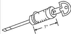
16-126 Key Cylinder
