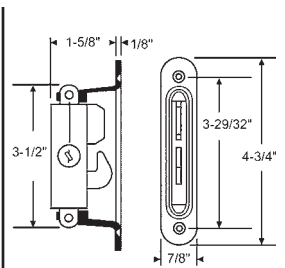
900-18867 Diagonal Hub. Aluminum Finish Use: 900-14560 for Keeper Traco
