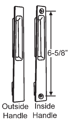
13-311 Flush mount dummy set. Chrome
