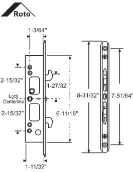
16-460 2-Point Patio Door Lock
