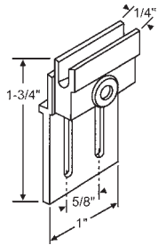
10-455 Aluminum Bracket w/Nylon Guide Croft
