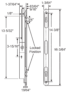
16-440W With Trimplate
