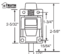
900-10574 Snap-on Vent Lock
