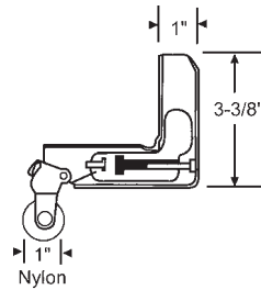
10-355 Maximum Corner Thickness 11/32" Jim Walters
