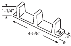
8-208 One Piece Nylon with Fixed Guides for 1-3/8" By-Passing Doors
