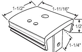
8-645 Mirror Door Guide & Bracket. Flexible Plastic Top Guide w/ Steel Mounting Bracket Monarch
