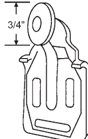
900-21054 3/4" Offset 900-21054S for Hanger w/Screws
