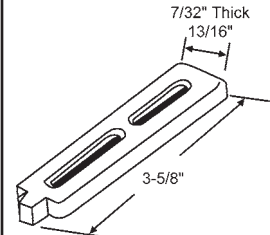
8-295 Guide Stem Paniflex
