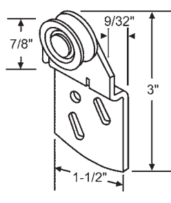
3-107 9/32" Offset 3-107S for Hanger with Screws
