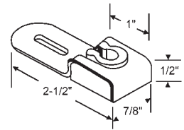
7-212 Metal with Nylon Insert
