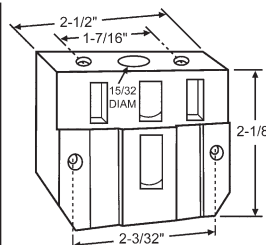
8-647 Corner Connector for Mirror Door
