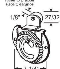
3-199 1/16" Offset Old Stanley
