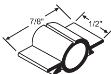
8-634 Tension Clip
