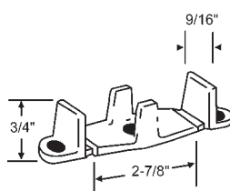
8-240 Nylon, White. Adjusts for Doors 3/4" - 1-3/4" E-Z Roll
