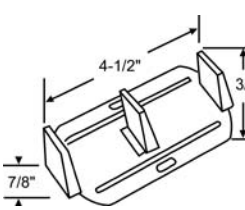
8-315 Metal with Nylon Posts For 1-3/4" Doors
