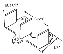
900-8114 Nylon 1 Piece. Fits 1-3/8" Doors
