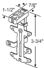
3-228 Guide Bracket
