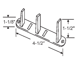
8-330 Metal with Nylon Posts Adjusts for Doors 3/4" - 1-3/8"
