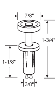
2-104 Top Rolling Guide Spring Loaded
