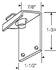
8-326 Adapter Plate
