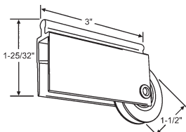
900-8319 Round-top Mirror Door Roller. Nylon Wheel
