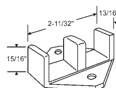
8-314 1 Piece. Floor Guide to Fit 3/4" Doors
