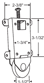
3-348 Wardrobe Door Bottom Roller with Angled Tang. Nylon Wheel
