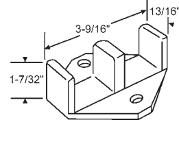
8-291 1 Piece. Floor Guide to Fit 1-3/8" Double Doors 1-1/4" High from Floor E-Z Roll
