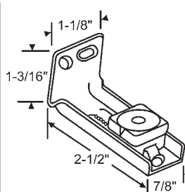
7-241 Metal with Nylon Insert
