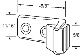
8-224 Metal Angle Stop w/Rubber Bumper Stanley
