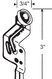
3-203 3/4" Offset w/ Screws
