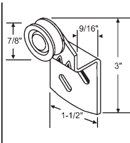
3-108 9/16" Offset 3-108S for Hanger with Screws
