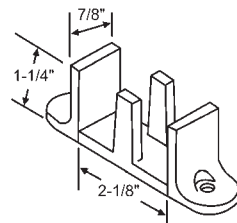
8-245 Adjusts for Doors 7/8" - 1-7/8" Nylon
