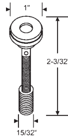
2-112 Top Rolling Guide 1" Round Nylon Wheel 2" Threaded Stem (For replacing older hardware)
