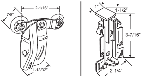
900-656 Front Dual Wheel Hanger
