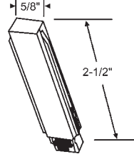
8-296 Nylon Insert Guide
