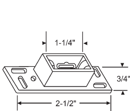
45-7 Drawer guide Old KD-07
