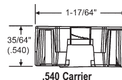
.540 Carrier
