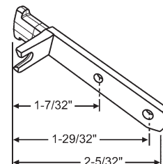
96CQ-30 Quick Tilt Pivot Bar
