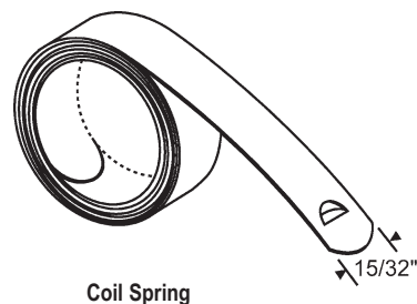
Coil Spring
