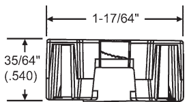
.540 Carrier
