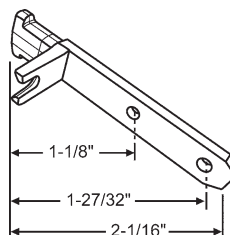
96CQ-29 Quick Tilt Pivot Bar
