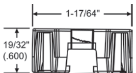
.600 Carrier
