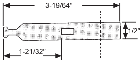
STANDARD SPRING
