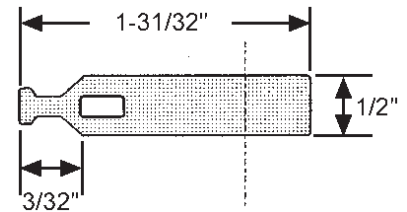
EGRESS SPRING
