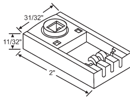
83-511 Opening: 9/32" x 7/32"
