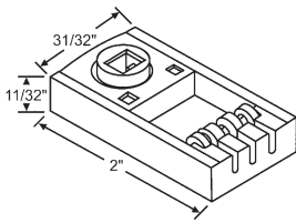
83-510 Opening: 9/32" x 7/32"
