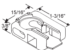
64T-500 Terminal Housing
