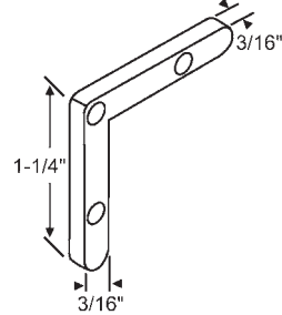
900-2229 Universal Nylon
