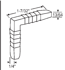
900-2278 Natural Nylon
