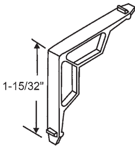
900-2251 Nylon
