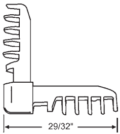
46-269 White Nylon
