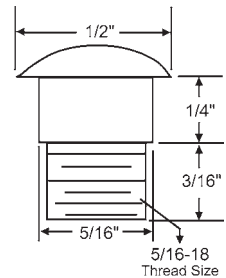
900-8530 Shoulder Bolt
