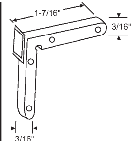
900-2209 Universal Nylon
