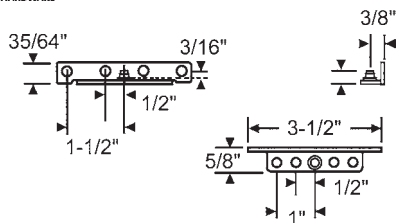
39-418 Non-Hand Snap Stud Bracket
