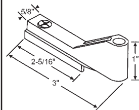
900-20957 Metal Bracket
