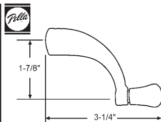
Fits Roto Operators 36-333SP, 36-334SP 5/16" Hex
