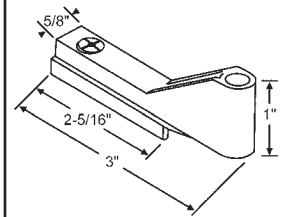
900-20957 Metal Bracket
