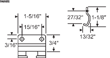
39-241 Center Hook for Lever Operator
