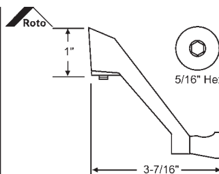
Folding Handle For Roto Pro Drive Operators
