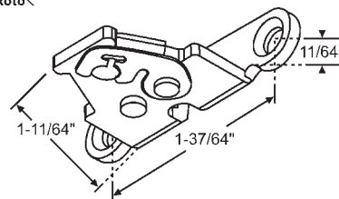
Sash Bracket for 750-1361484
