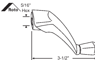
For X-Drive Operators. Other Finishes Available.
