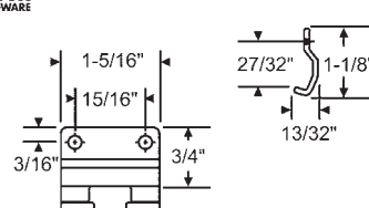
39-241 Center Hook for Lever Operator
